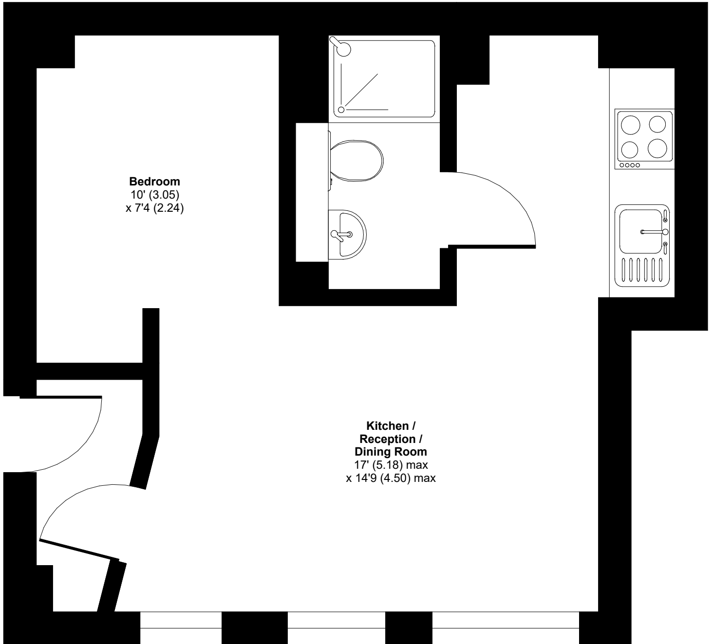
THIRD FLOOR
